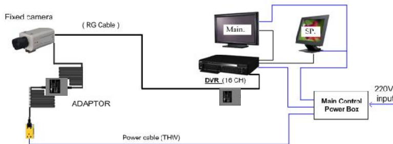
CCTV. system diagram
