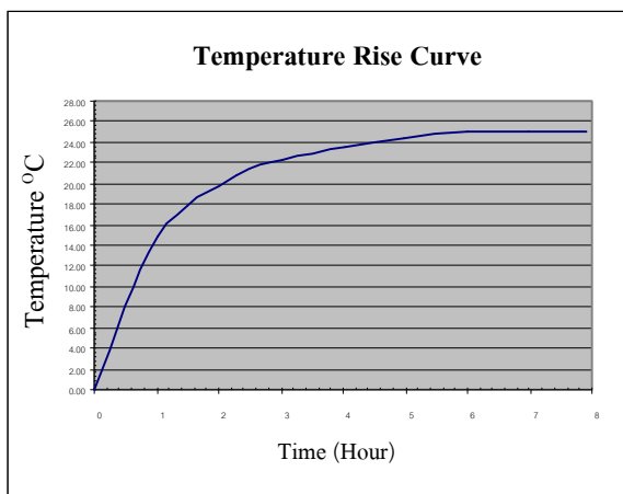
Model: CV-02 On 25 °C Ambient
