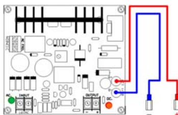
Power supply Board (Open frame)
